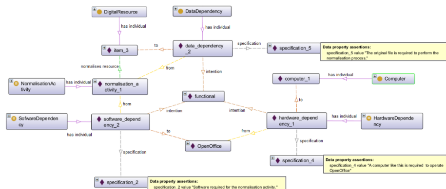
Fig. 1. All three types of dependencies combined together to attribute a complicated scenario of dependencies with functional intention.
